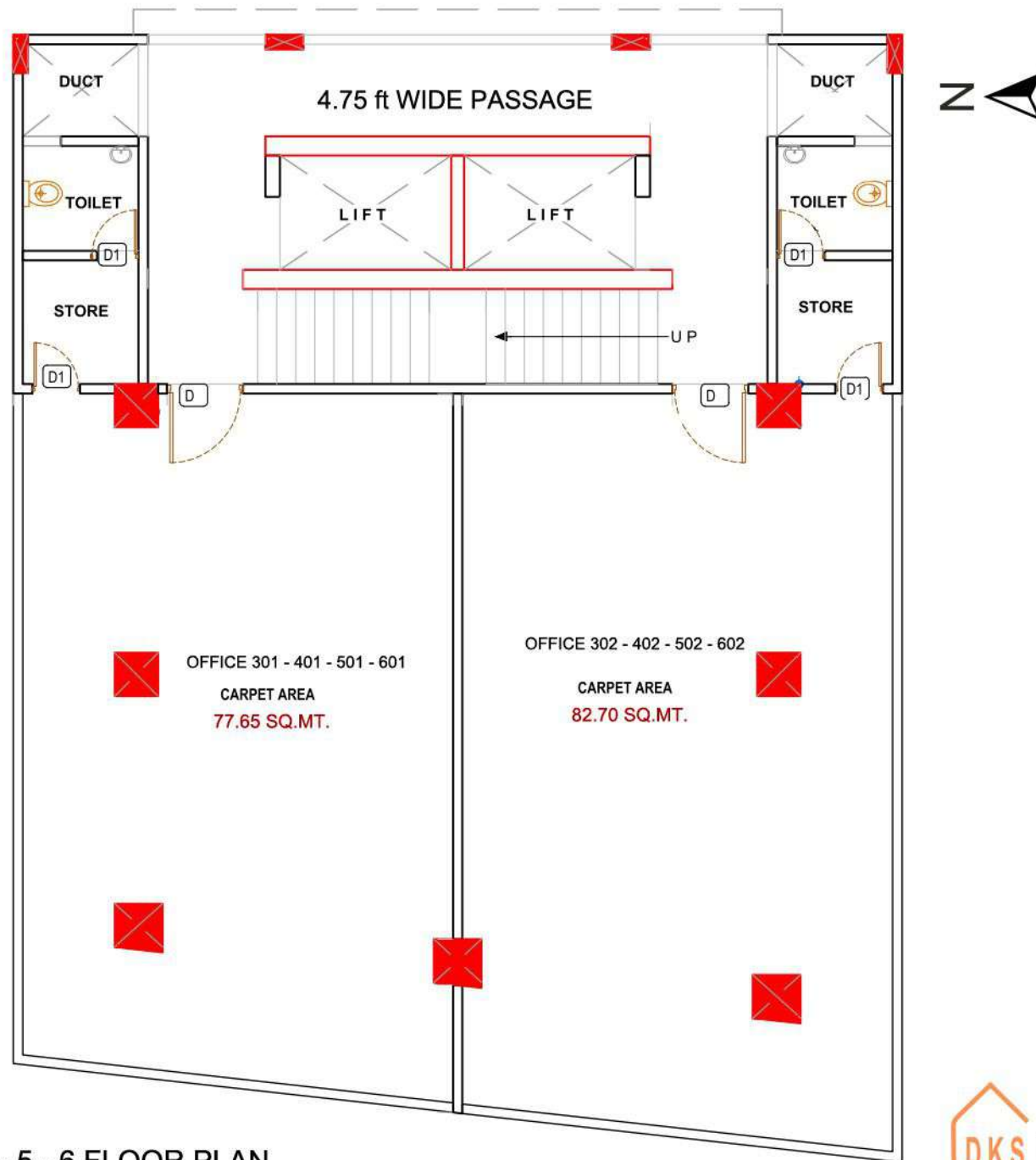
3 - 4 - 5 - 6 FLOOR PLAN
