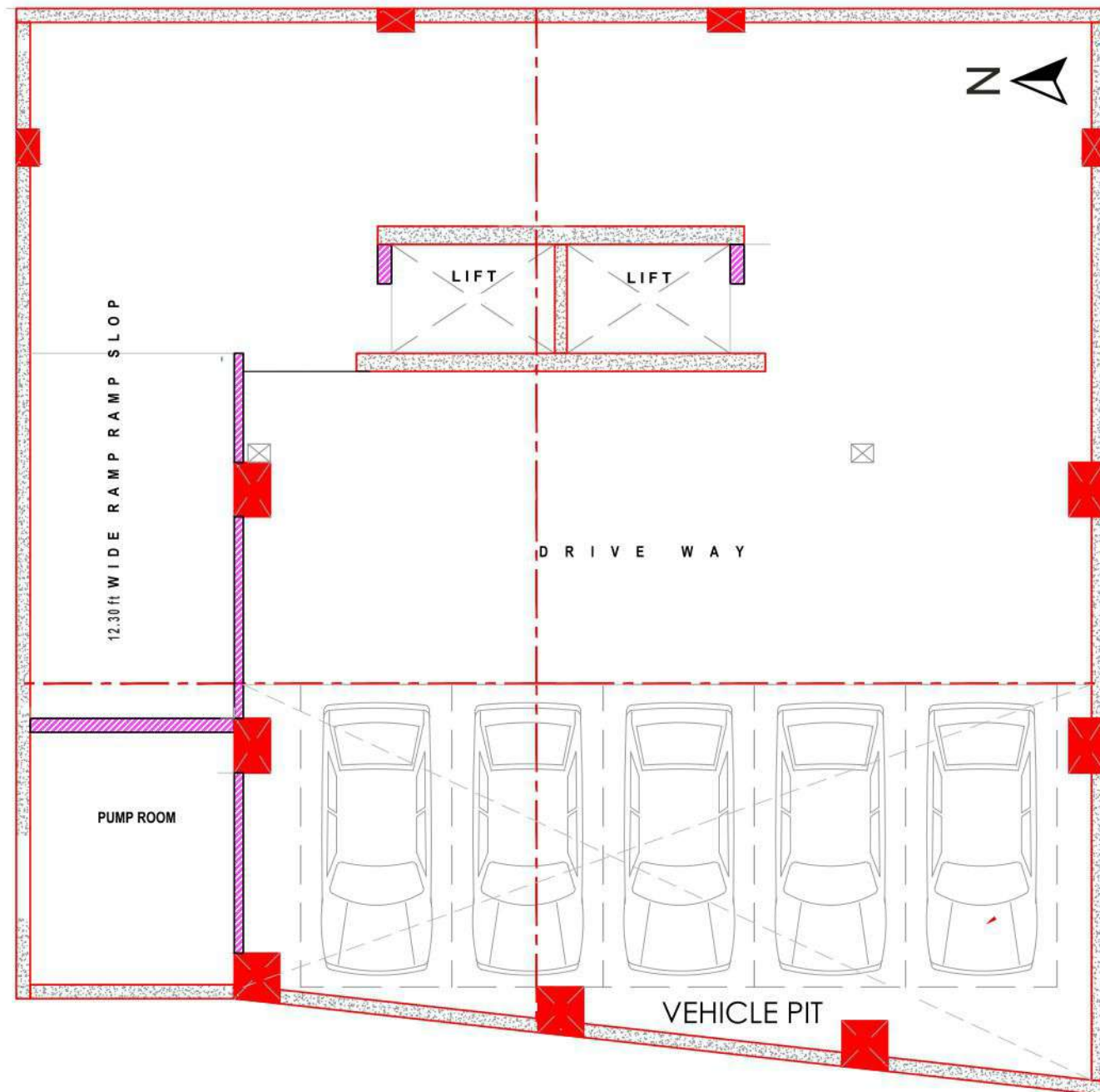
BASEMENT PLAN
